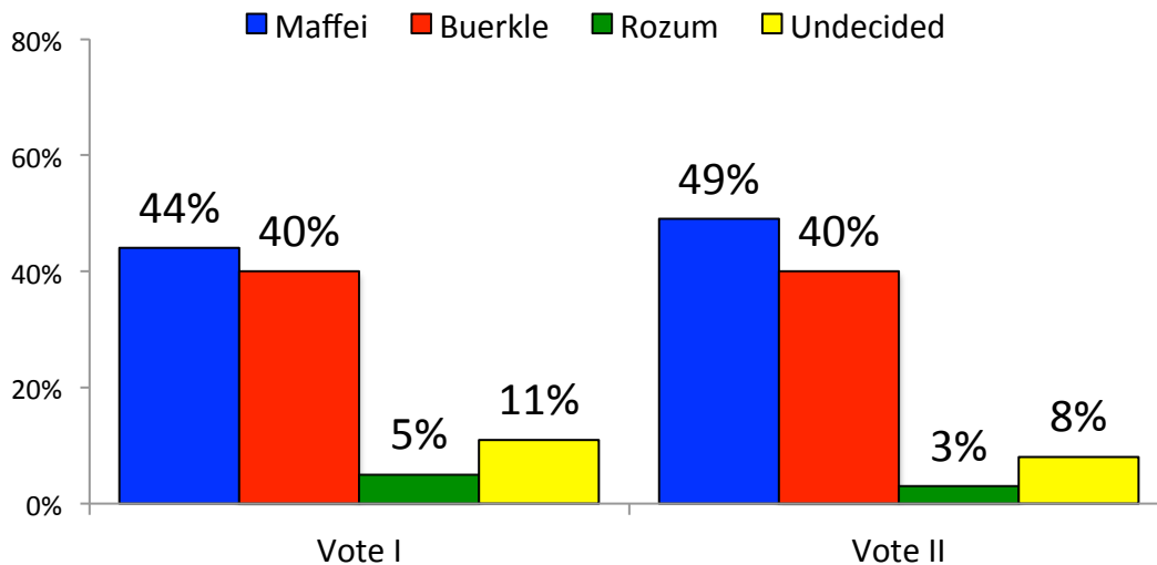
Initial Vote for U.S. Congress and Vote After Positive Paragraphs Maffei expands his lead to 9 points
